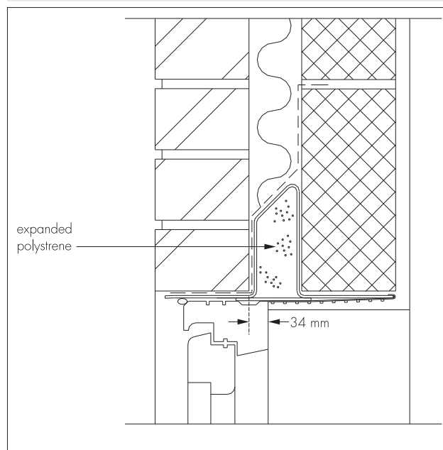
Figure 2 Installation detail — L1/HD 50
