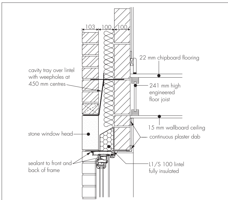
Figure 4 Installation detail – L1/S 100 (100 mm cavity/partial fill)
