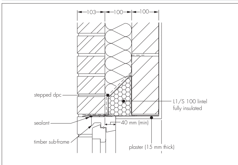
Figure 3 Installation detail — L1/S 100 (100 mm cavity/full fill)
