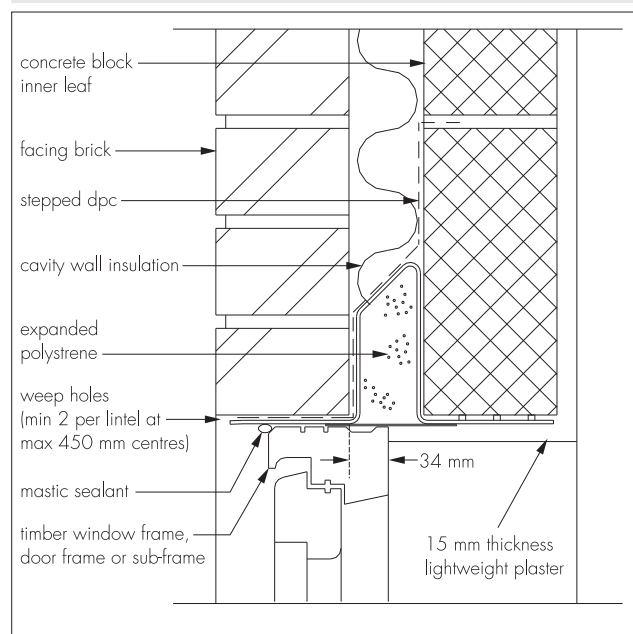
Figure 1 Installation details — L1/S 50
