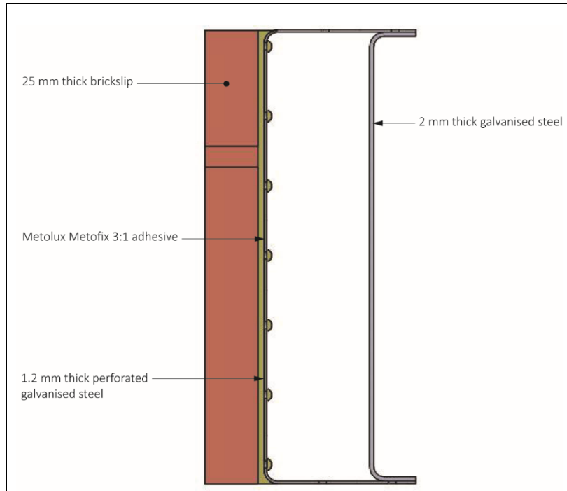
Figure 1 Components of Lightweight Brick Slip Feature Lintels and Sills
