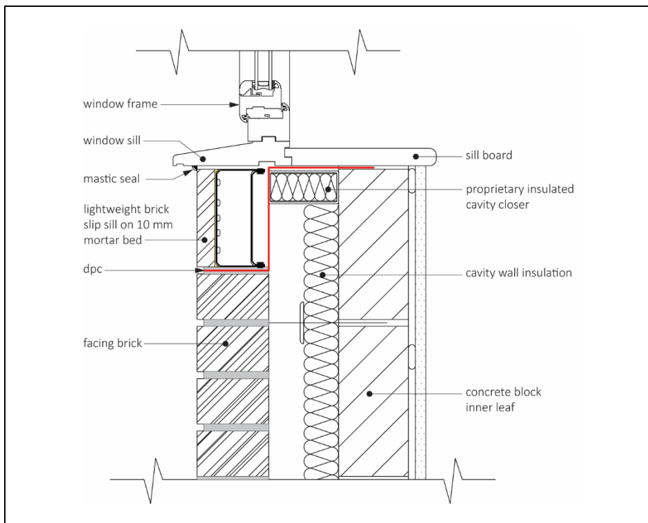
Figure 5 General cross-section of Lightweight Brick Slip Feature Sills
