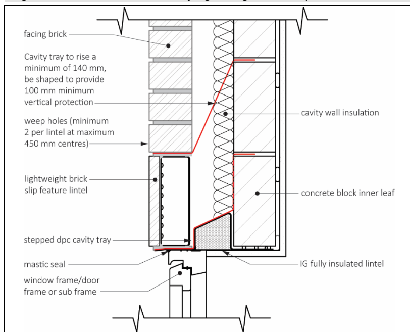
Figure 2 General cross-section of Lightweight Brick Slip Feature Lintels
